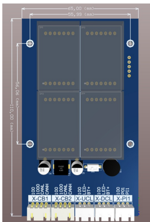
Figure 3: BC-D4X Mounting Dimensions
