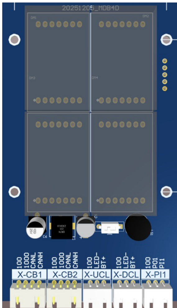
Figure 1: Front 3D View of the BC-D4X
